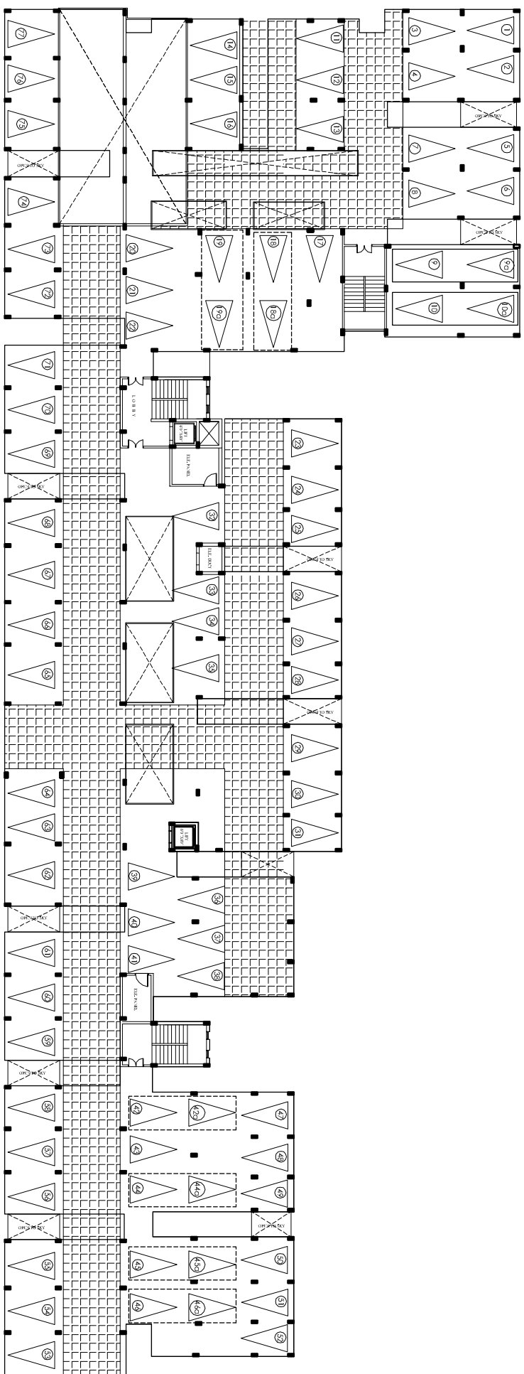
G-BLOCK STILT PARKING PLAN
