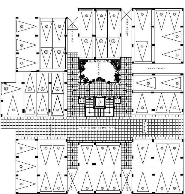
F-BLOCK STILT PARKING PLAN
