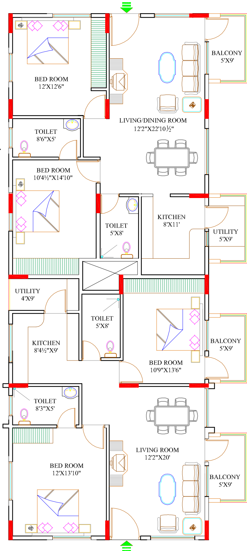
TYPE-G 2 BEDROOM - 1,200 Sft.
